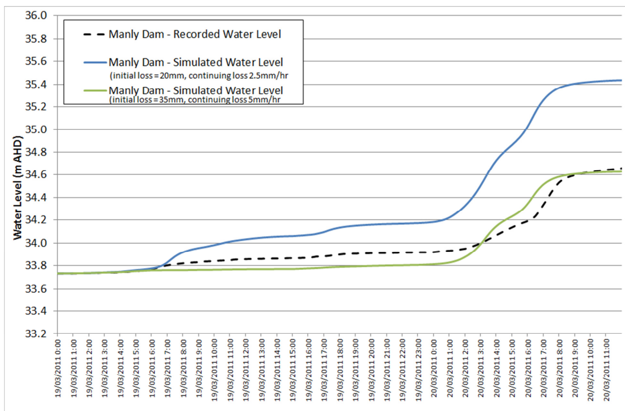
Figure 5-11 Manly Dam Water Level Calibration – March 2011
