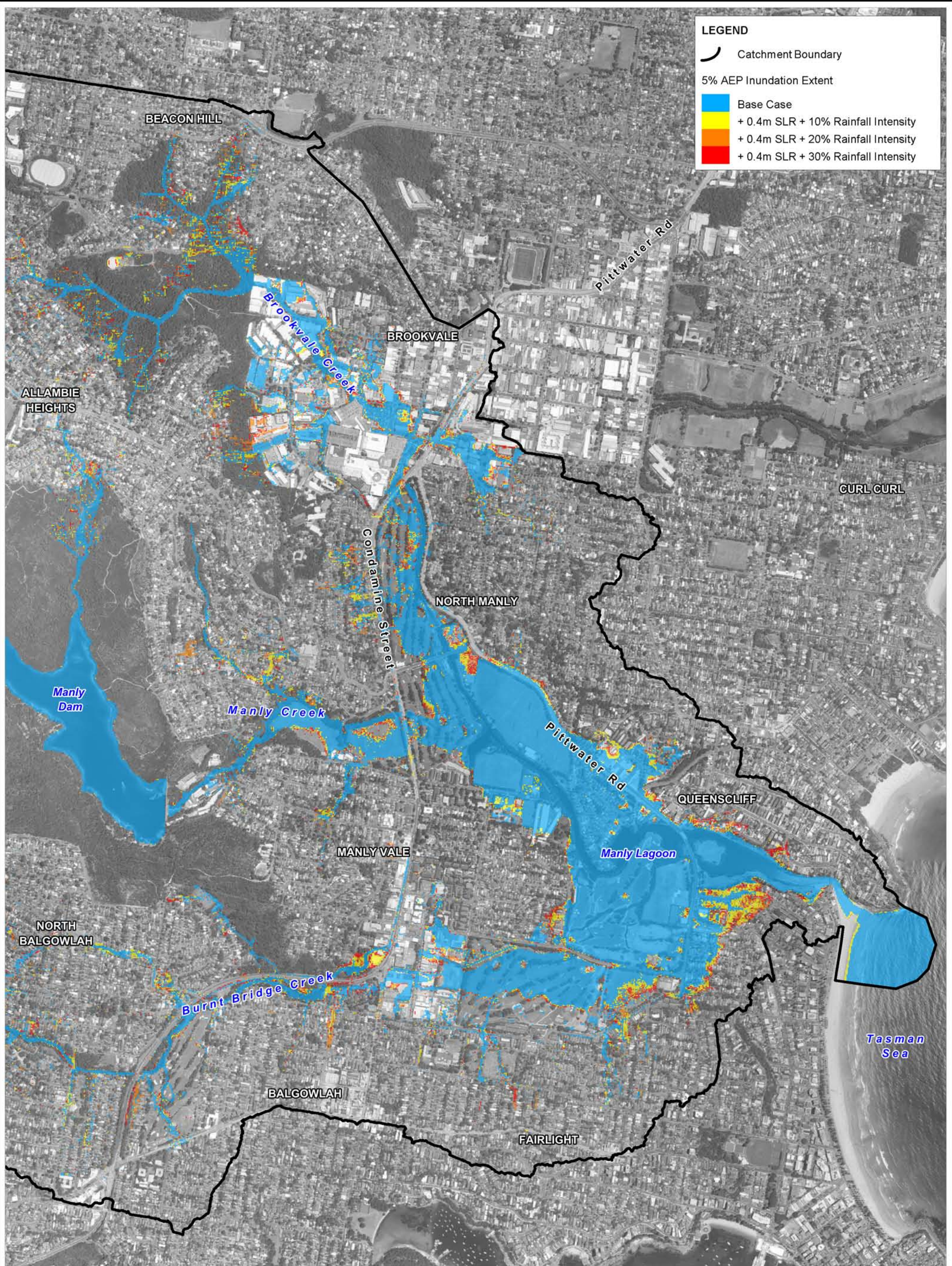
Title: Manly Lagoon Flood Study - Climate Change Scenarios: 5% AEP Catchment Derived Event + 0.4 m SLR + Rainfall Intensity Increase
