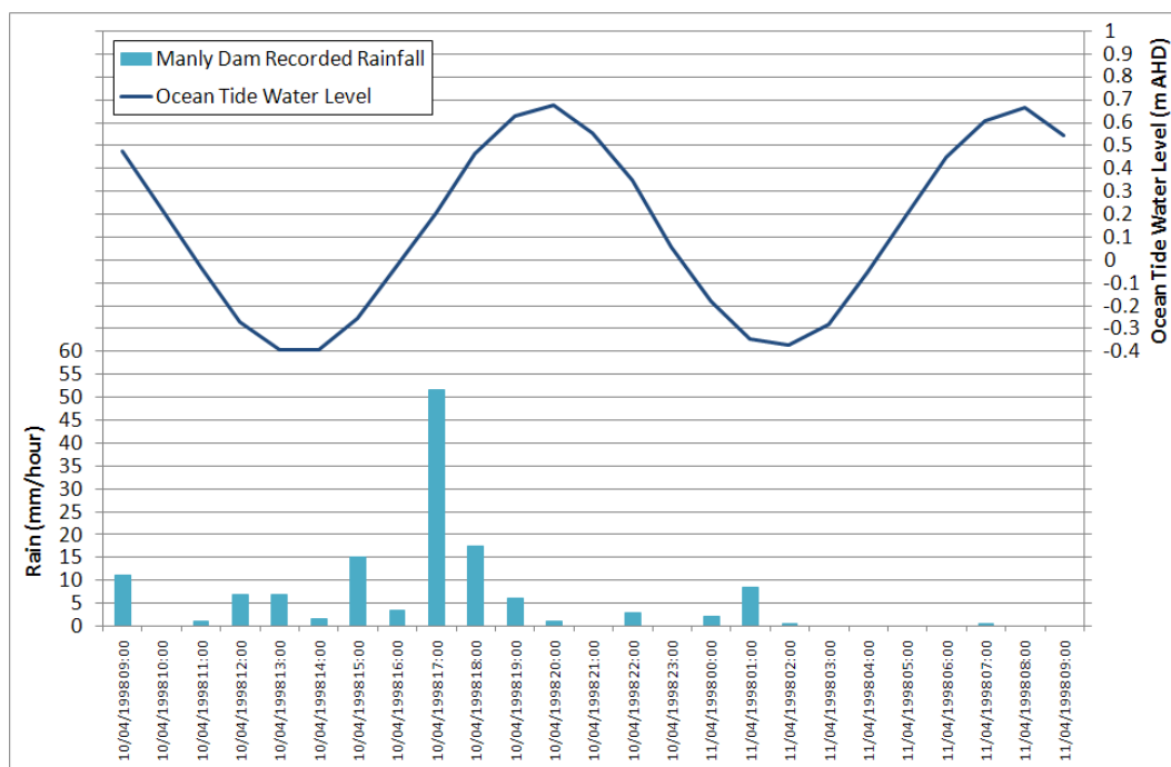
Figure 5-17 April 1998 Recorded Tidal Water Level
