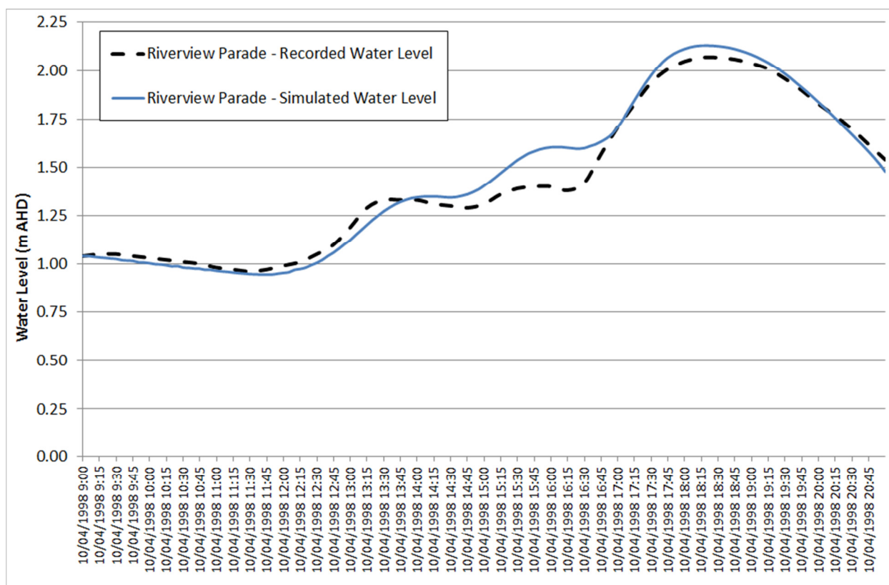
Figure 5-19 Riverview Parade Water Level Calibration – April 1998
