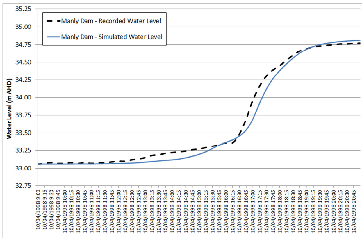
Figure 5-21 Manly Dam Water Level Calibration – April 1998
