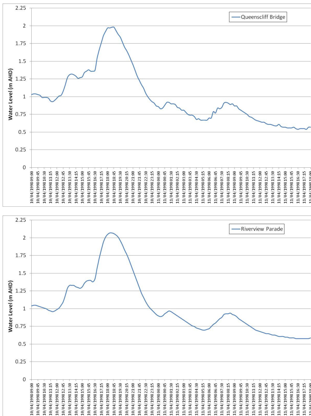
Figure 5-15 April 1998 Recorded Water Levels at Manly Lagoon
