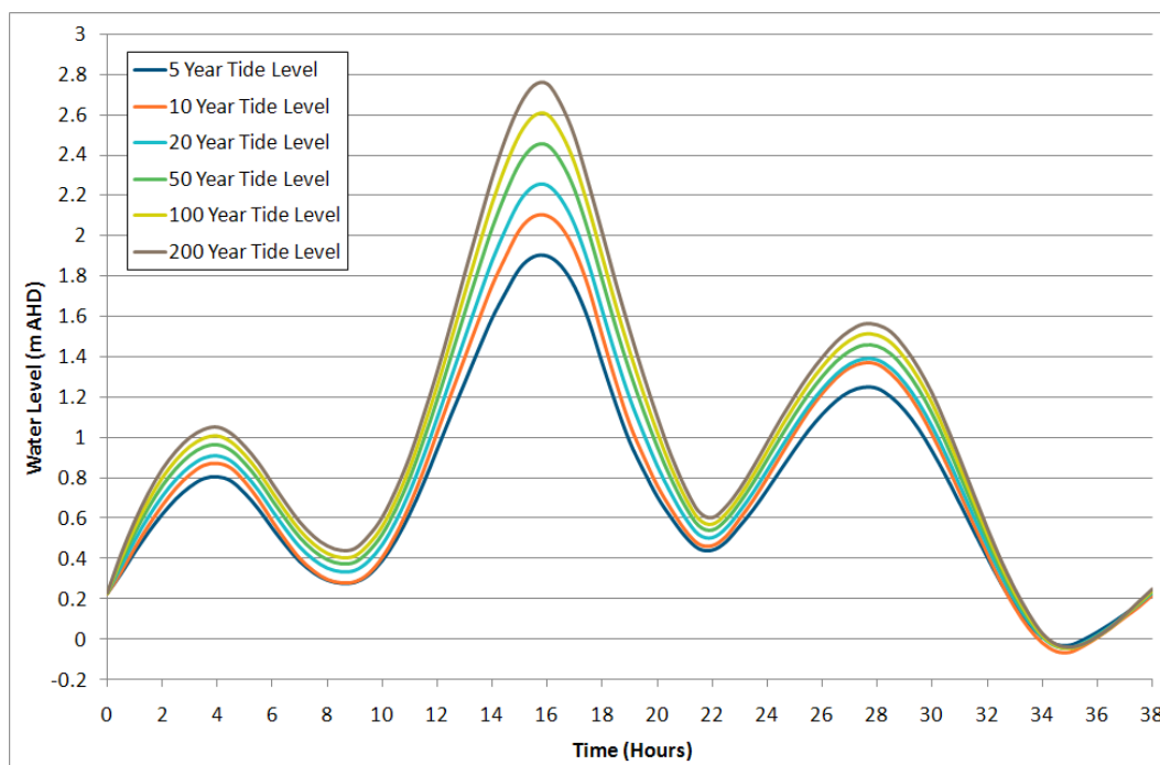
Figure 6-3 Design Ocean Boundary – Elevated Tide
