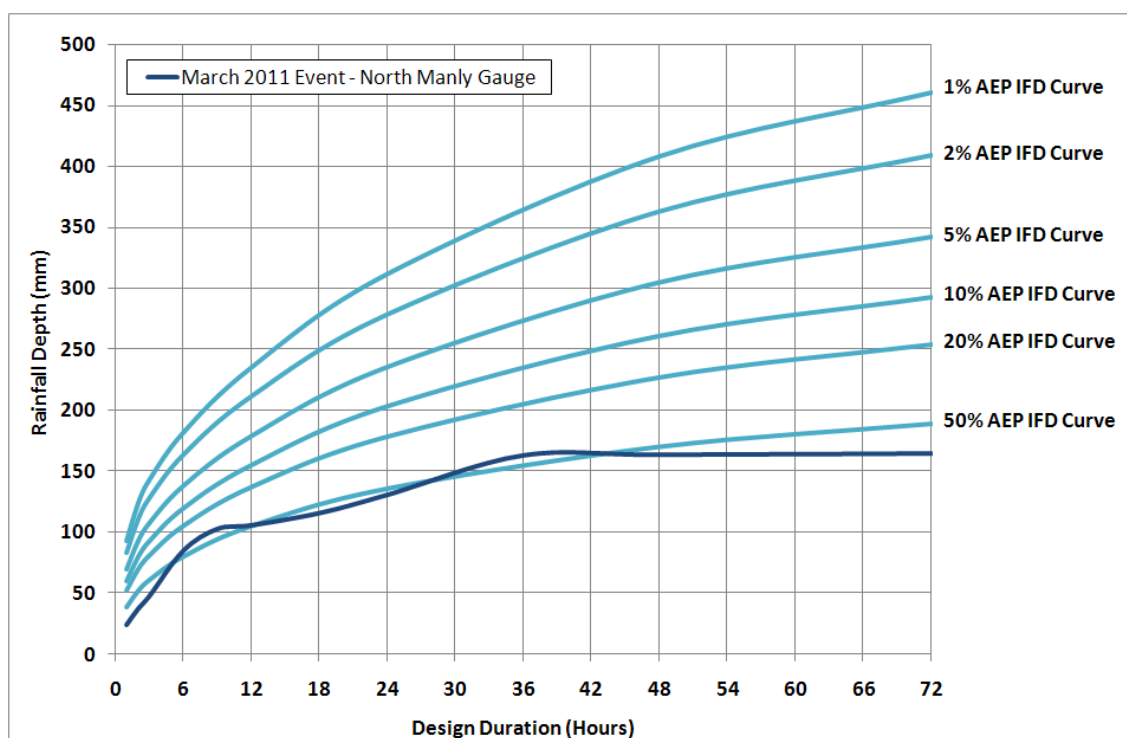
Figure 5-3 Comparison of March 2011 Rainfall with IFD Relationships
