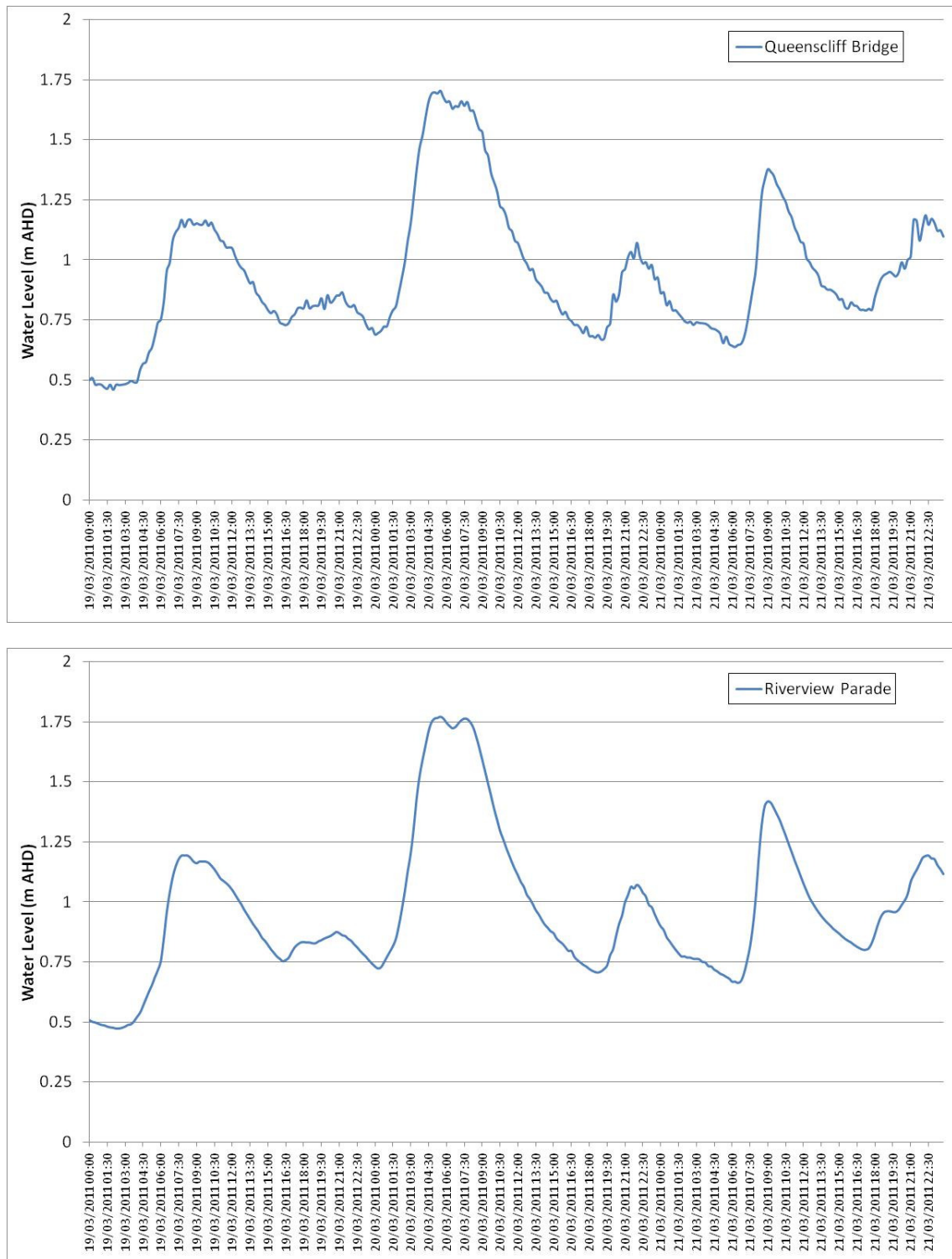
Figure 5-4 March 2011 Recorded Water Levels at Manly Lagoon
