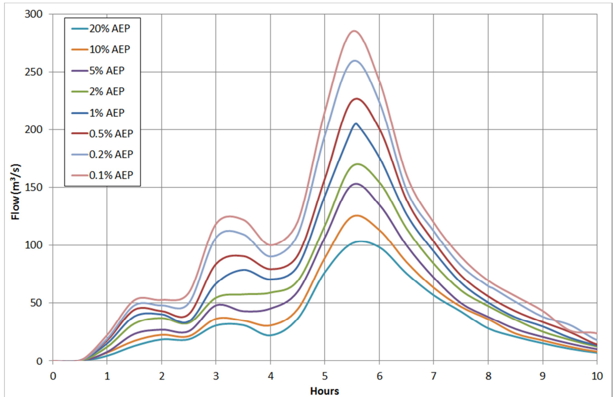
Figure 7-6 Combined Inflows to Manly Lagoon for Sample Design Events
