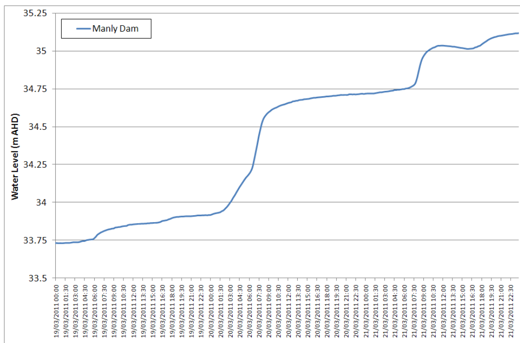
Figure 5-5 March 2011 Recorded Water Levels at Manly Dam
