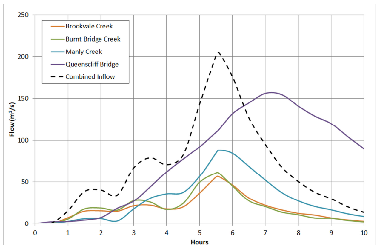
Figure 7-5 Sub-catchment Contributions to Manly Lagoon (1% AEP Event)
