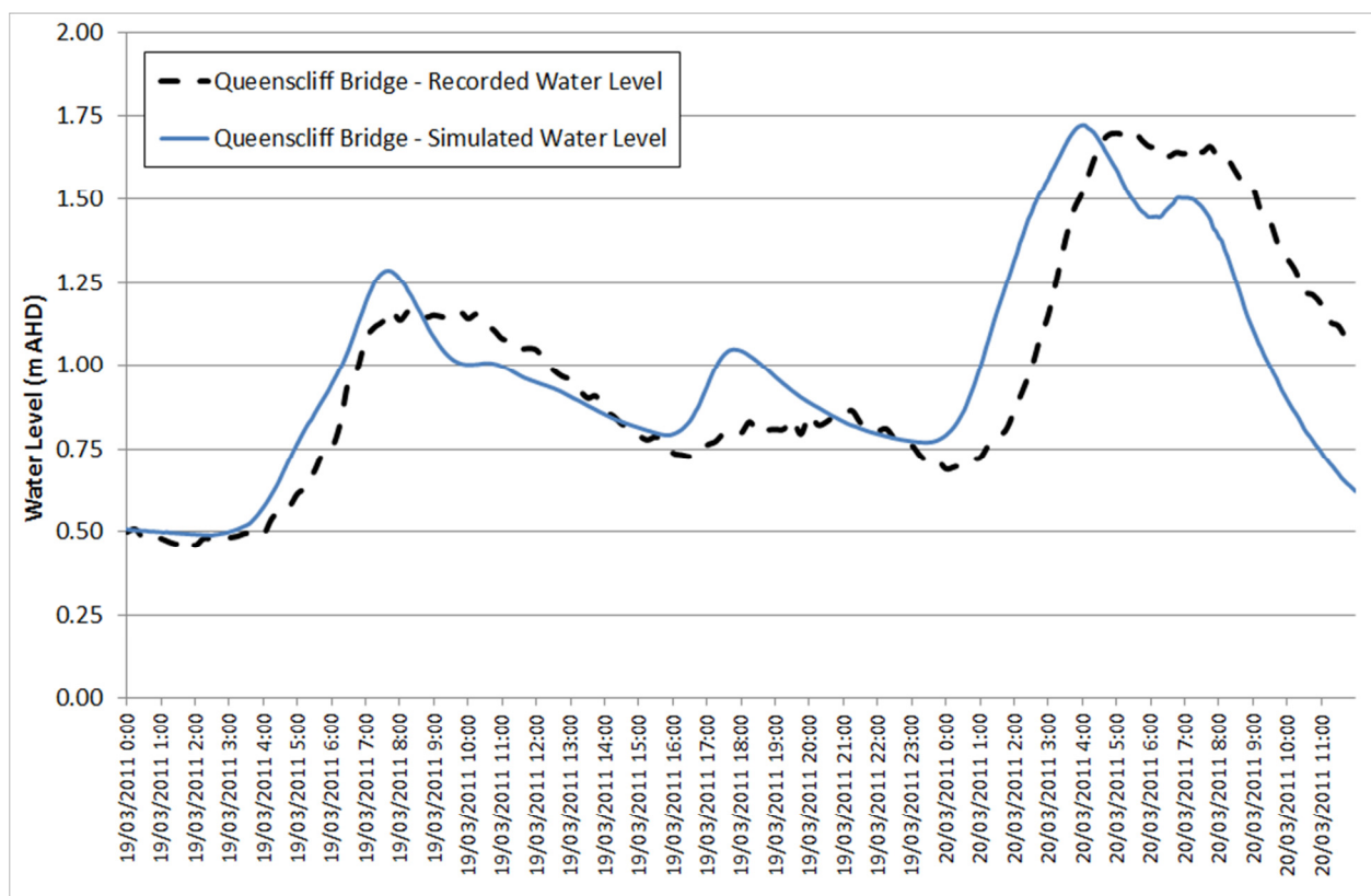
Figure 5-10 Queenscliff Bridge Water Level Calibration – March 2011
