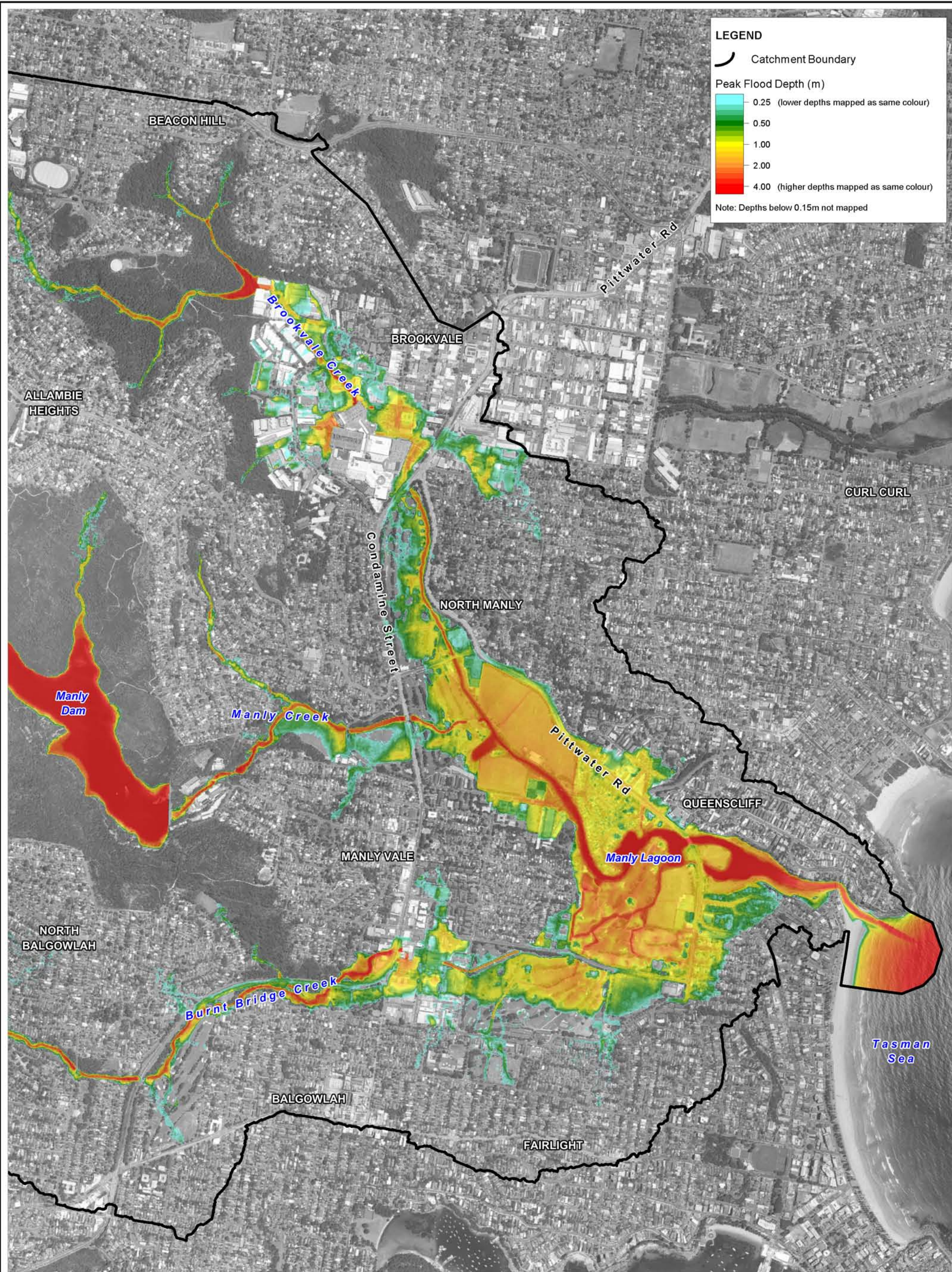
Title: Manly Lagoon Flood Study - Peak Flood Depths: 0.2% AEP Catchment Derived Event
