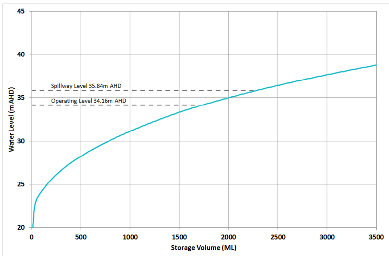
Figure 4-5 Manly Dam Stage-Storage Relationship
