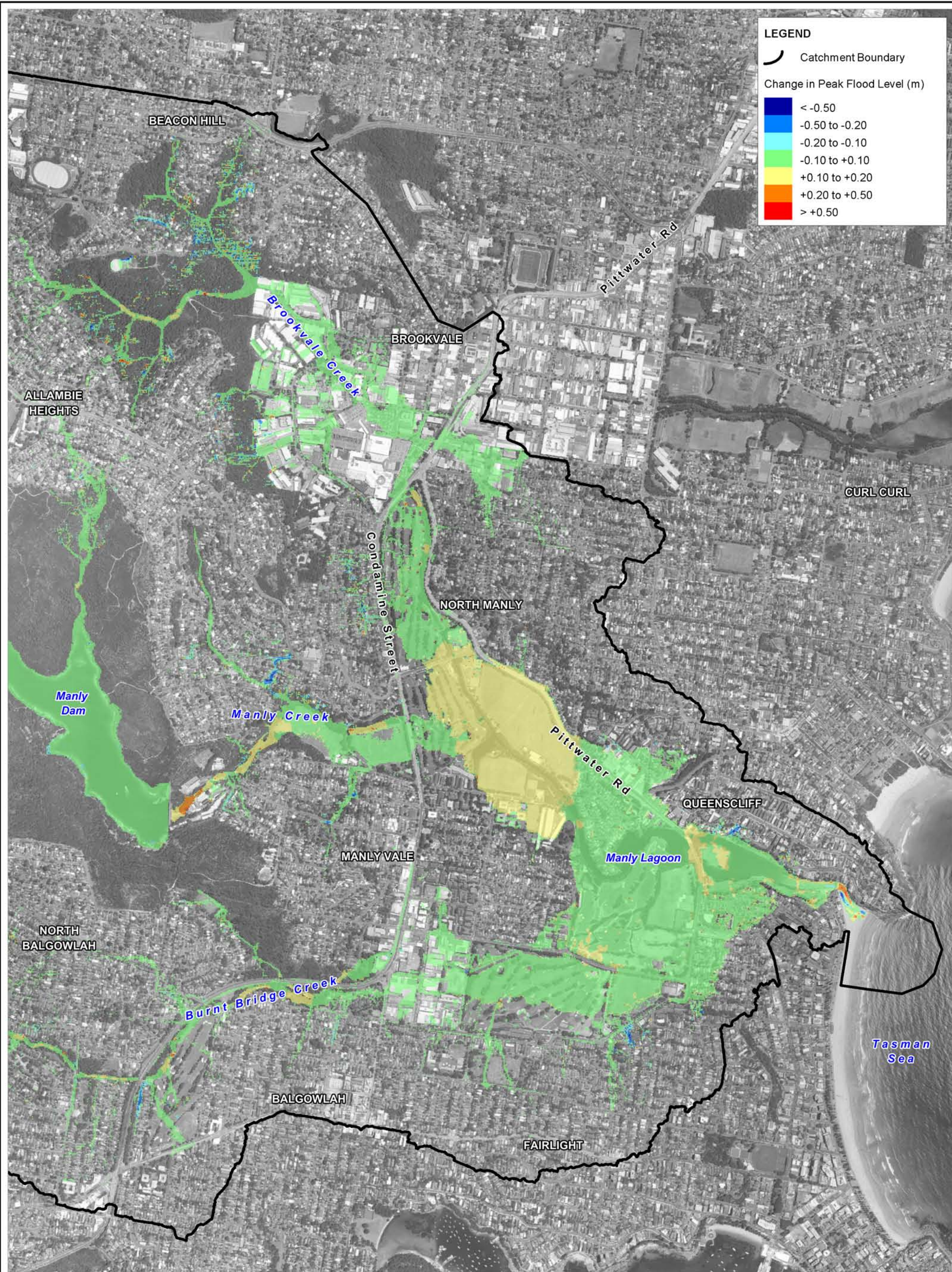
Title: Manly Lagoon Flood Study - Change in Peak Flood Level: Increased Hydraulic Roughness (1% AEP Catchment Derived Event)
