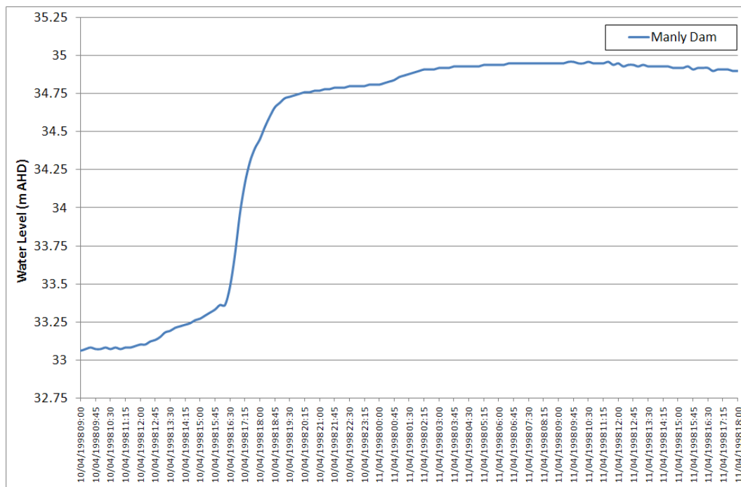
Figure 5-16 April 1998 Recorded Water Levels at Manly Dam
