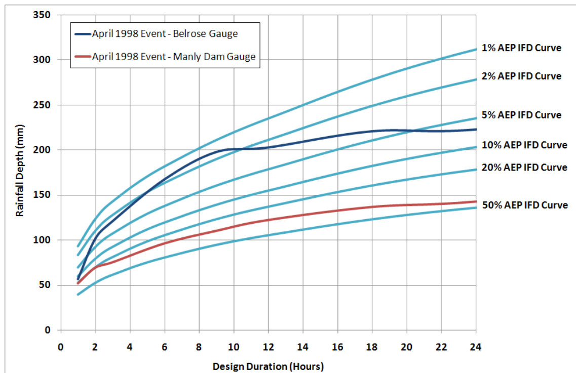
Figure 5-14 Comparison of April 1998 Rainfall with IFD Relationships
