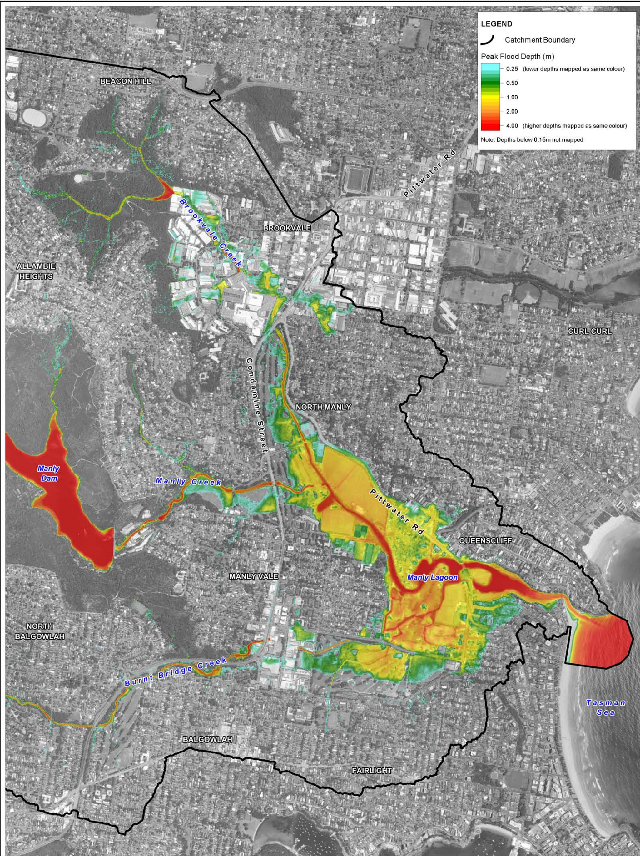
Title: Manly Lagoon Flood Study - Peak Flood Depths: 1% AEP Catchment + 5% AEP Ocean Coincident Event
