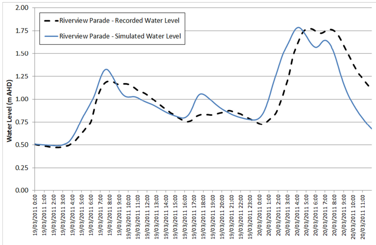
Figure 5-9 Riverview Parade Water Level Calibration – March 2011
