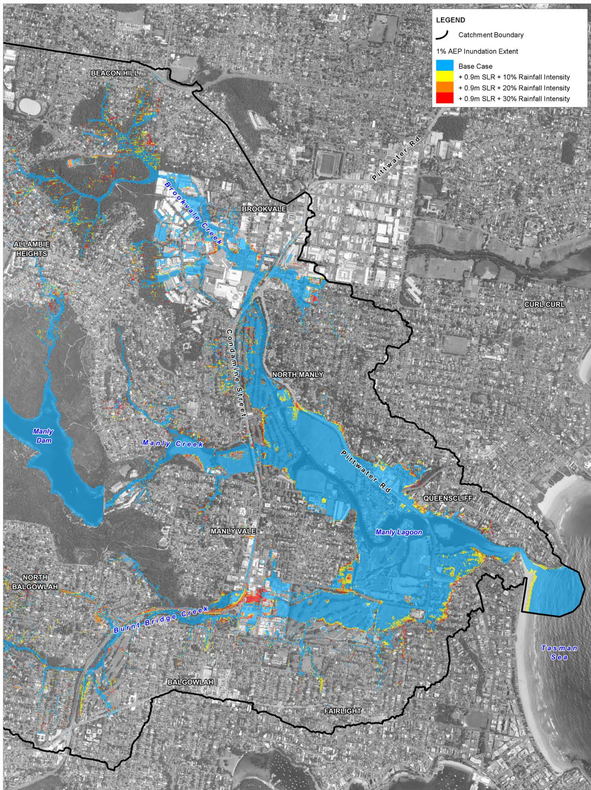
Title: Manly Lagoon Flood Study - Climate Change Scenarios: 1% AEP Catchment Derived Event + 0.9 m SLR + Rainfall Intensity Increase
