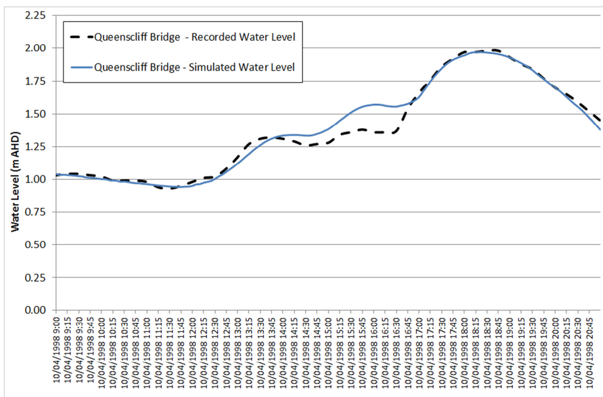
Figure 5-20 Queenscliff Bridge Water Level Calibration – April 1998
