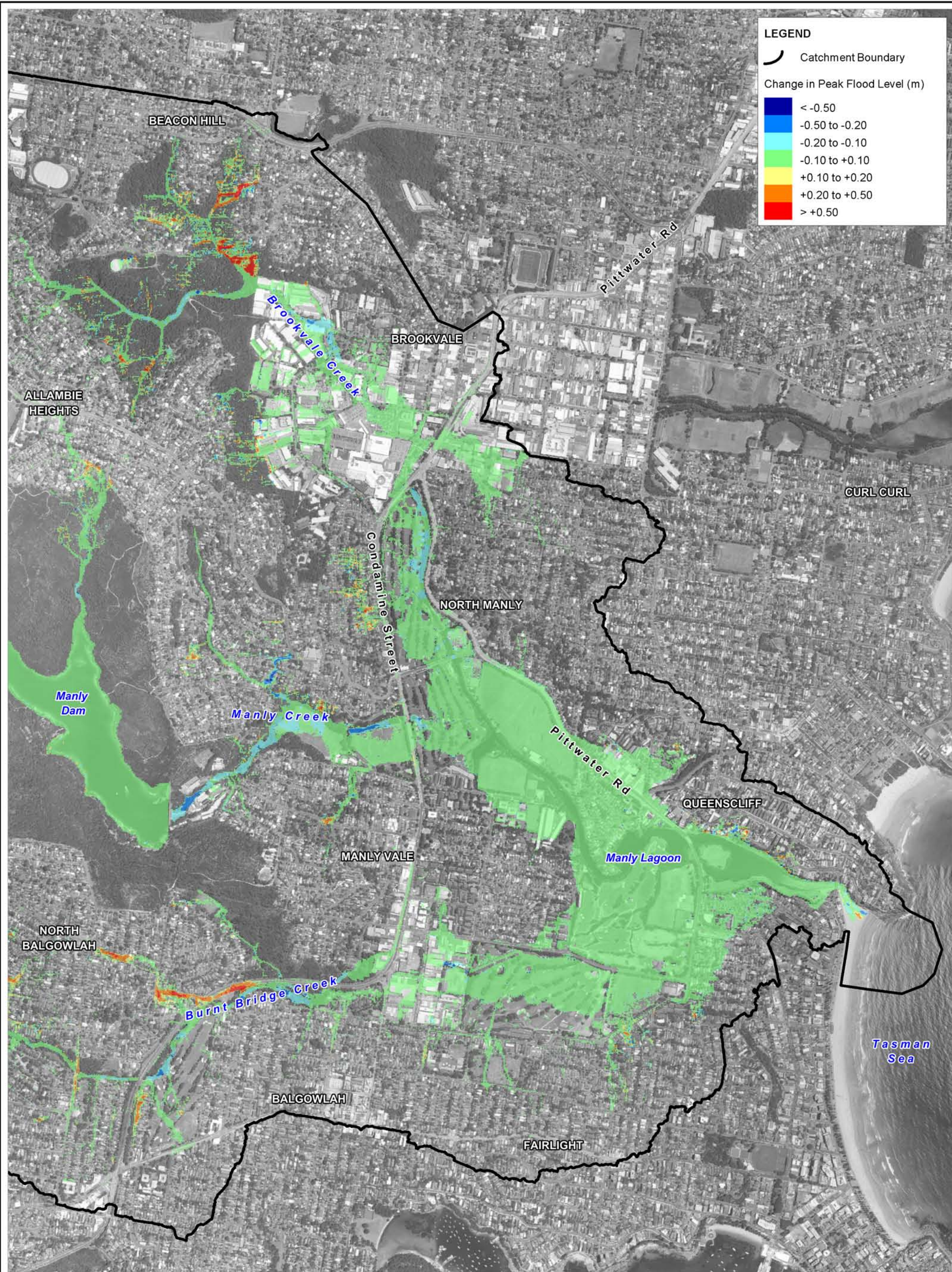
Title: Manly Lagoon Flood Study - Change in Peak Flood Level: Decreased Hydraulic Roughness (1% AEP Catchment Derived Event)
